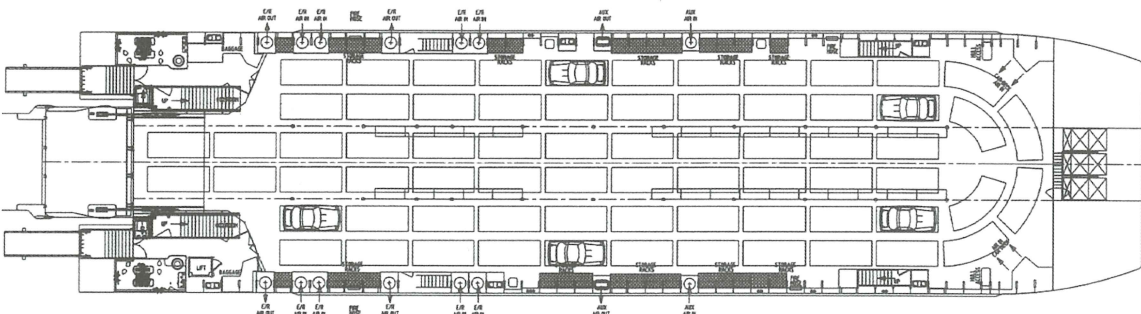
MAIN DECK
