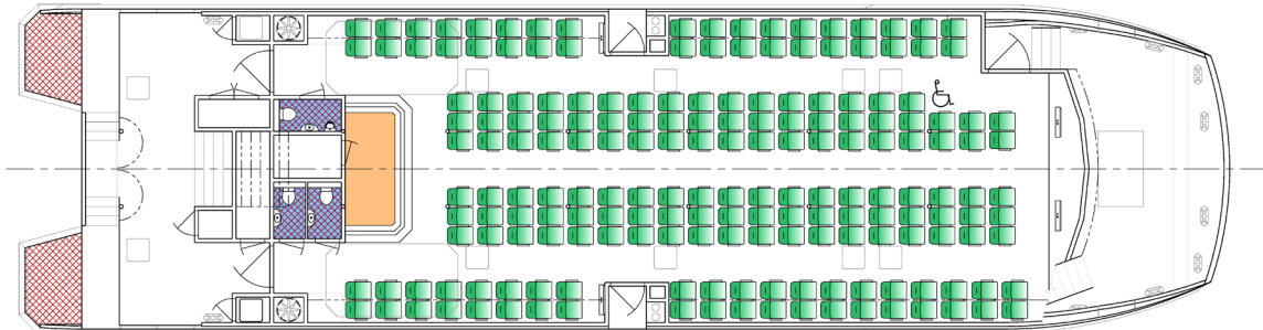
MAIN DECK
