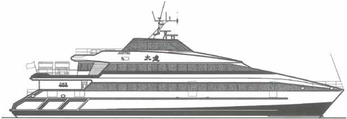
PROFILE
