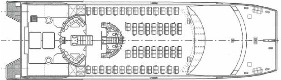
UPPER DECK
