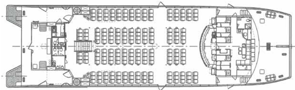
MAIN DECK
